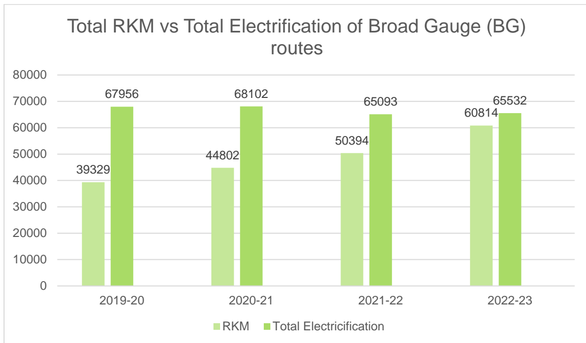
Figure 84: Route electrification in Indian Railways 123
