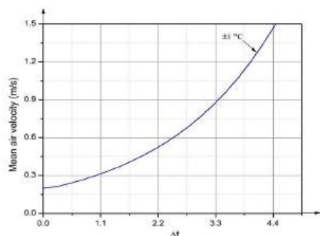
Figure 11.1: Required Air Speed to Offset Increased Operative Temperature (in Celsius) Figure 11.1 and the example given below (based upon the methodology from ISO 7730) can be used to find increase in acceptable operative temperature at elevated air speed above 0.2 m/s.
